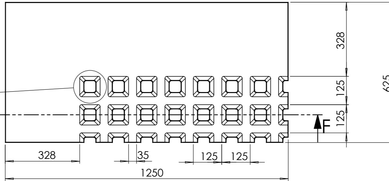
SECTION F-F
