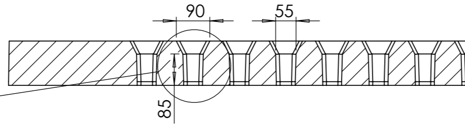
SECTION F-F
