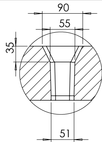
DETAIL C
