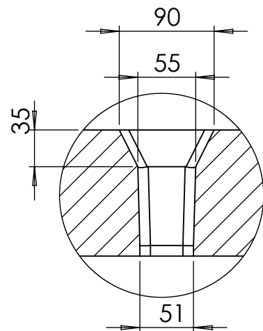
DETAIL C
